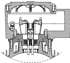
Terminal box for motor sizes 280 - 315
