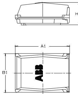
Motor sizes 355-400 side-mounted: 142/5, 142/10, 162/5, 162/8
