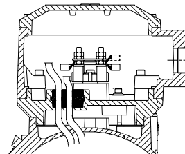
Terminal box for motor sizes 200 - 250
