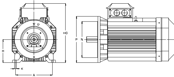
Flanges
