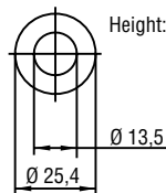
Ring magnet OD25,4 Part No. 400 533 Composite: PA-Ferrite Weigh ca. 10g Operating temperature: -40 ... +100°C
